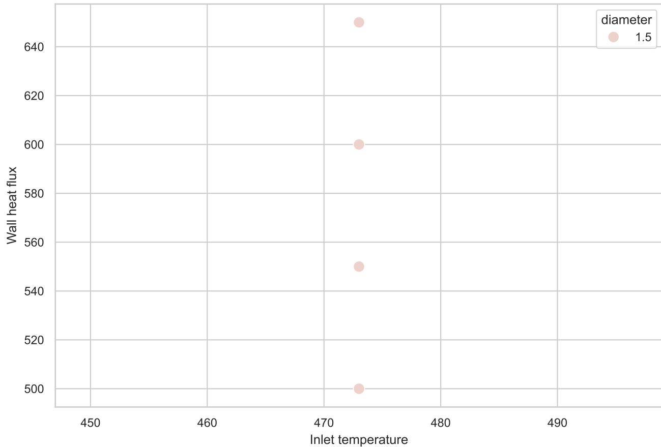
Case Matrix
