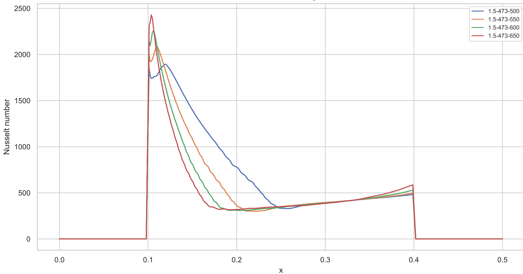
Nusselt number along x
