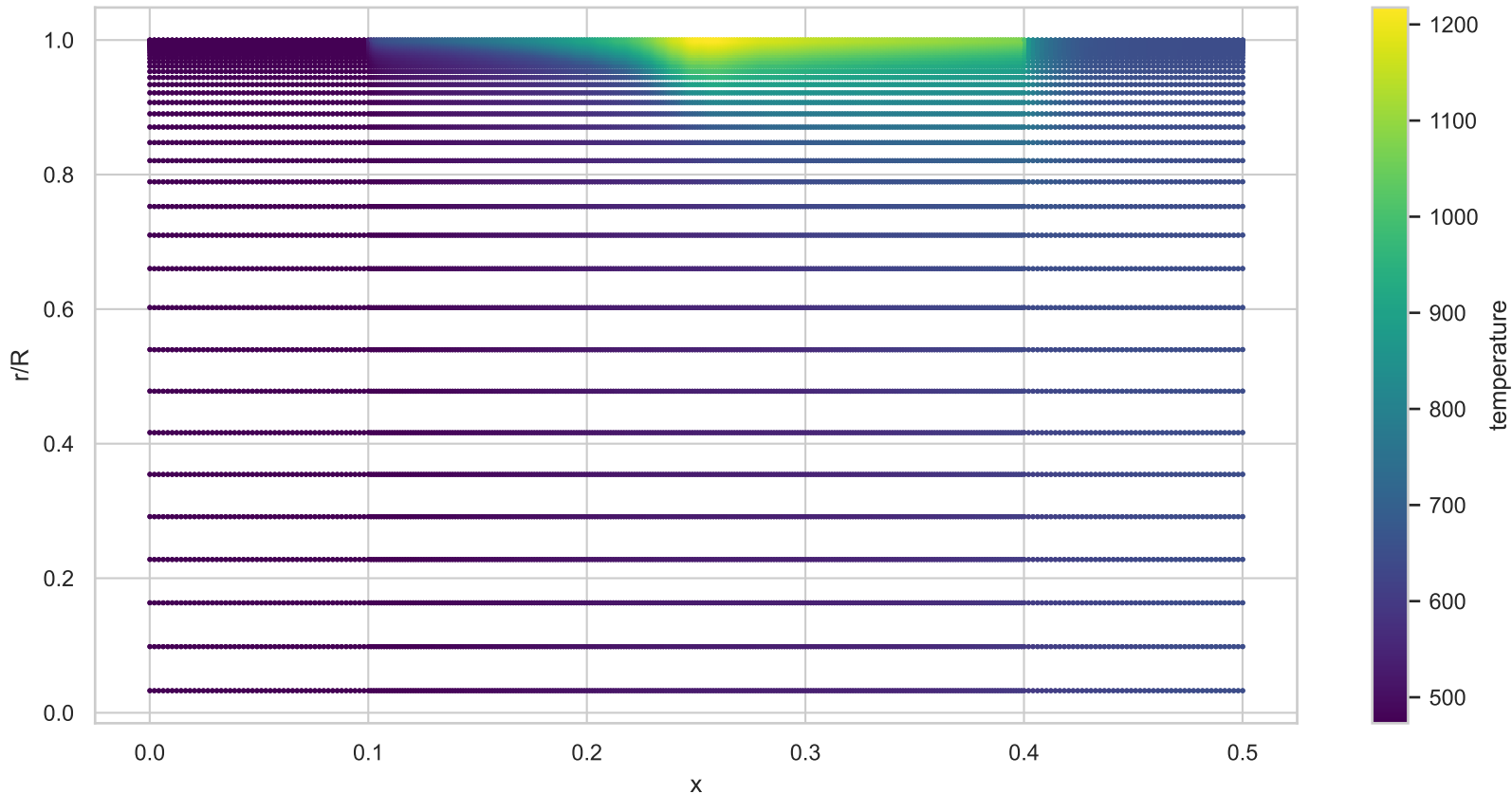
temperature cloud (1.5-473-500)
