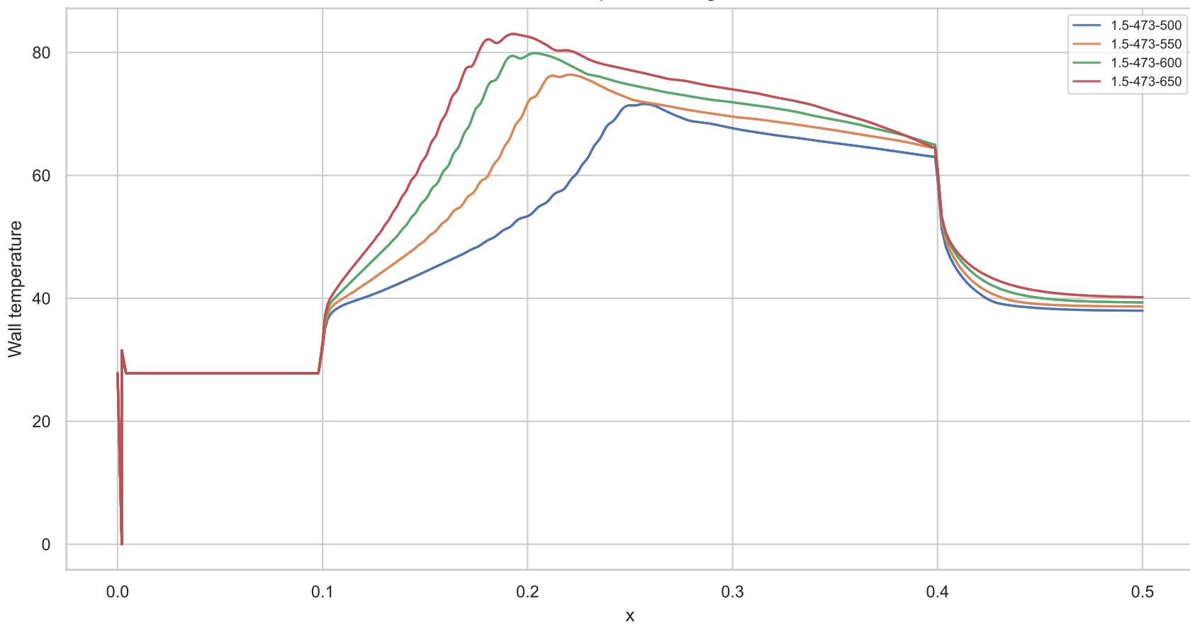
Wall temperature along x
