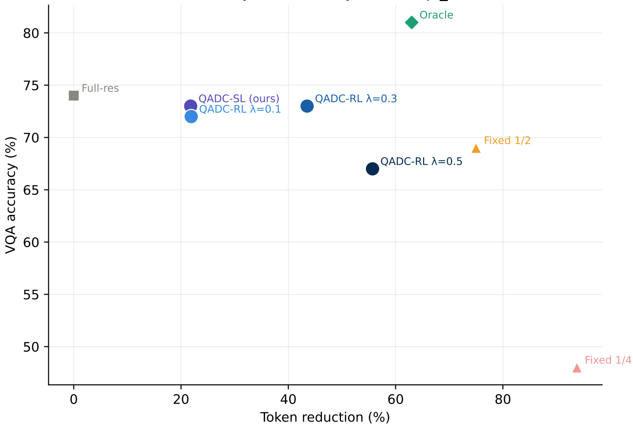
Accuracy vs Efficiency — textvqa_val
