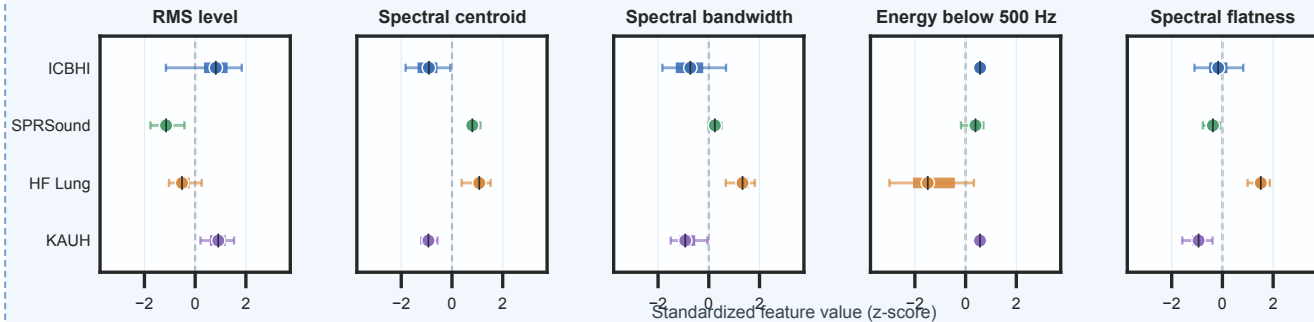
(c) Standardized acoustic feature distributions across balanced recording groups
