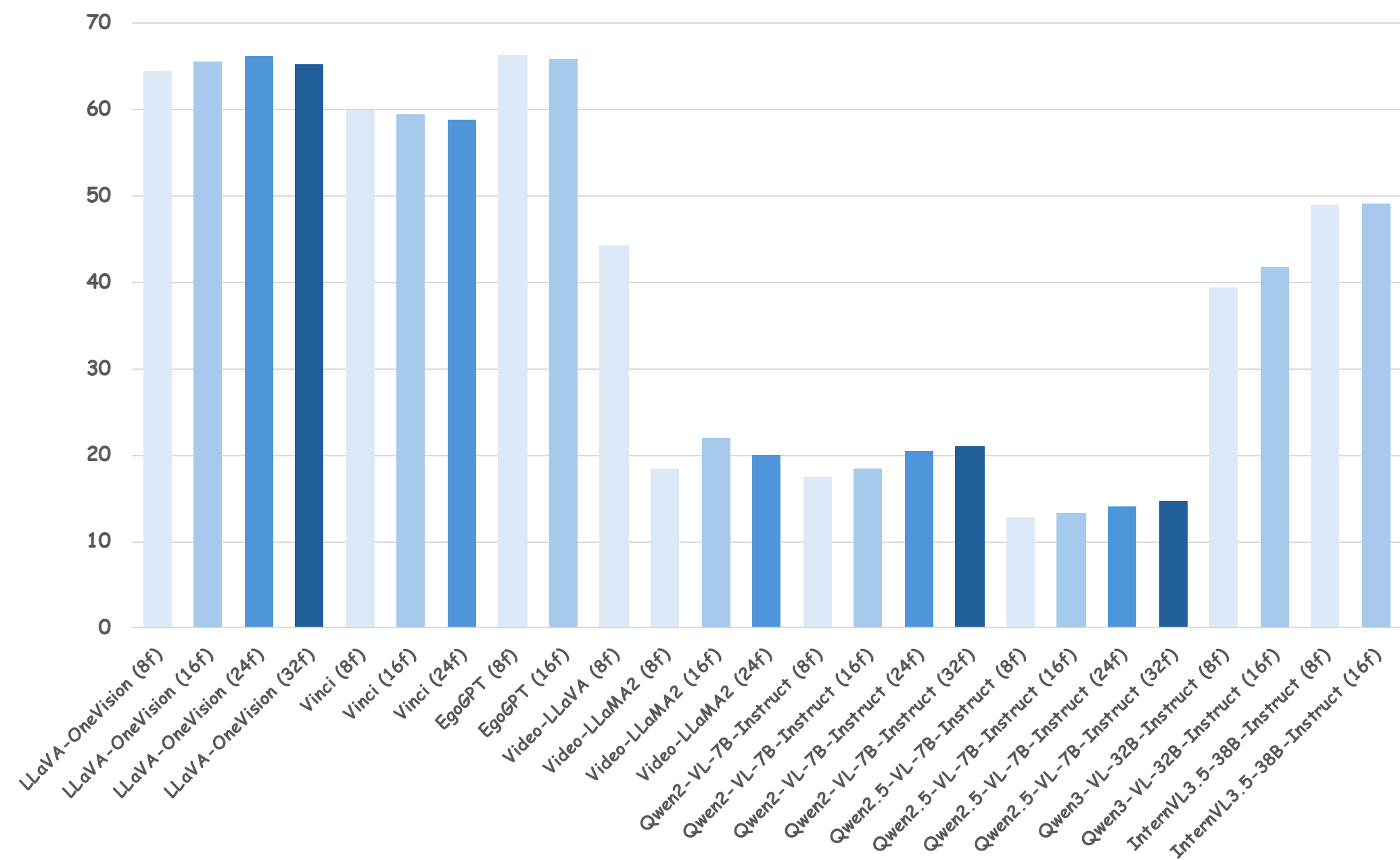
(a) Accuracy
