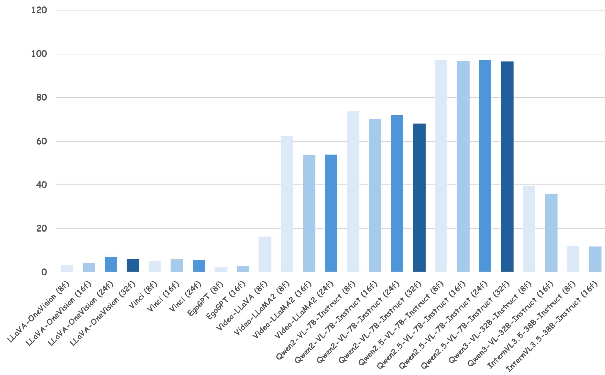
(c) Recall
