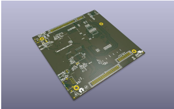
AM3352-OLinuXino Rev A (Olimex)
