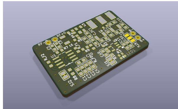
RTL-SDR direct-sampling differential amplifier (Z. Doczi)
