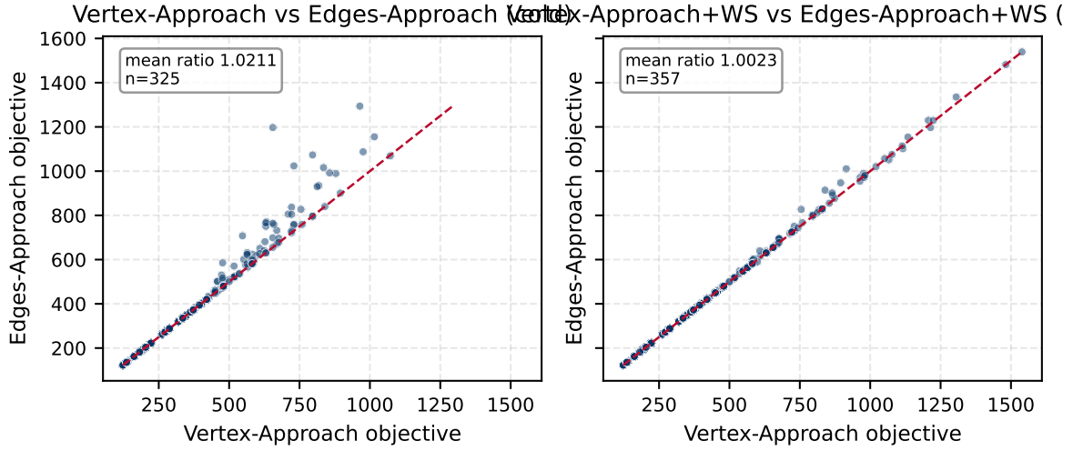
Figure 6: Objective parity check: Vertex-Approach (MTZ) vs. Edges-Approach (DFJ) on the 325 (cold) / 357 (warm) configs where both formulations finished. Diagonal = equivalence. Mean ratio Edges-Approach/Vertex-Approach = 1.021 (cold) and 1.002 (warm), confirming the two MIQPs are equivalent up to solver variability and time-limit effects; warm-start closes the residual gap.
