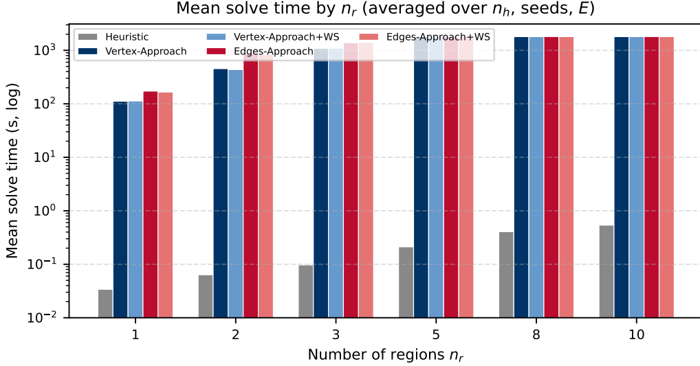
Figure 5: Mean solve time (log scale) vs. number of regions n_r , averaged over n_h , E and seeds. Vertex-based (Vertex-Approach, MTZ) vs. edge-based (Edges-Approach, DFJ lazy) with and without warm-start, plus heuristic, on the full testbed.
