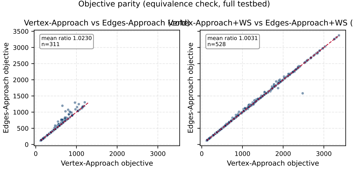
Figure 7: Objective parity check: Vertex-Approach (MTZ) vs. Edges-Approach (DFJ) on the 311 (cold) / 528 (warm) configs where both formulations produced a solution. Diagonal = equivalence. Mean ratio Edges-Approach/Vertex-Approach = 1.023 (cold) and 1.003 (warm), confirming the two MIQPs are equivalent up to solver variability and time-limit effects; warm-start closes the residual gap.
