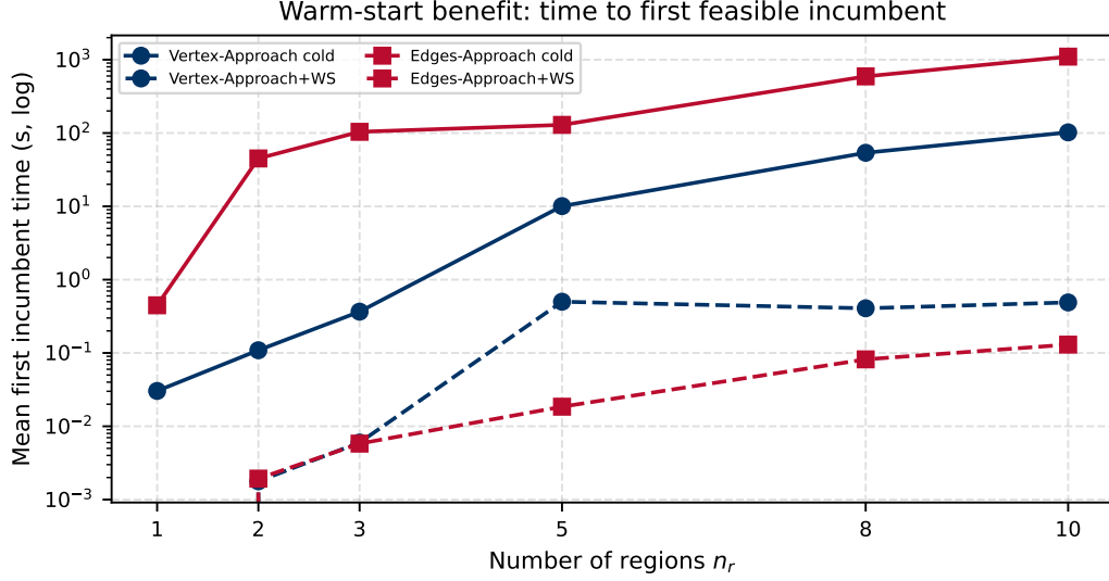
Figure 8: Time to first feasible incumbent (mean over seeds/ n_h/E ). Solid = cold start, dashed = warm-start. Warm-start reduces the time by one to two orders of magnitude, especially for tight endurances; the effect is visible for both Vertex-Approach and Edges-Approach.
