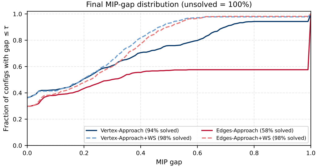
Figure 7: Distribution of final MIP gaps over the 540 configs (runs with no solution counted at 100%). Warm-starting shifts both formulations markedly left: the fraction under 50% gap rises from 76% to 93% (vertex) and from 57% to 90% (edges). Legend shows the fraction of configs solved by each method.
