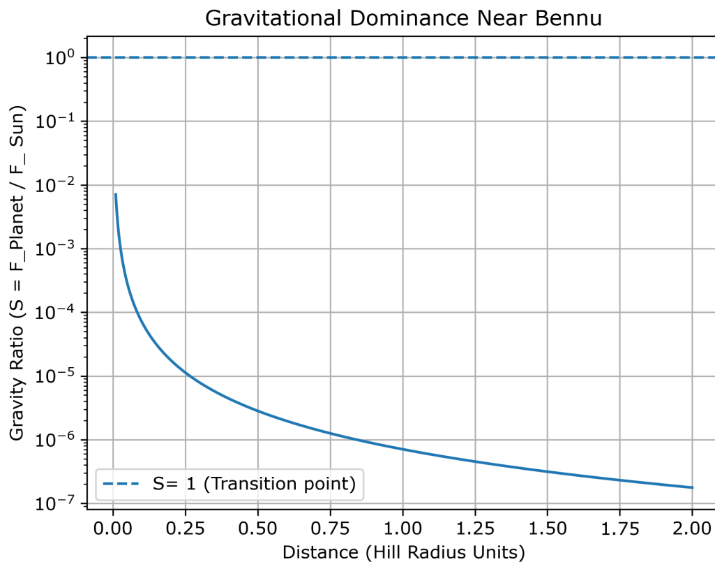
Figure 5. Stability profile for asteroid 101955 Bennu. No transition point is observed within the sampled range, indicating the absence of a dominant gravitational region.
