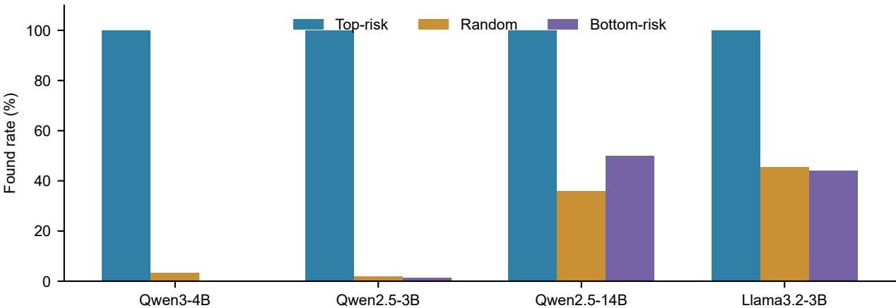
Same-budget layer-selection controls
