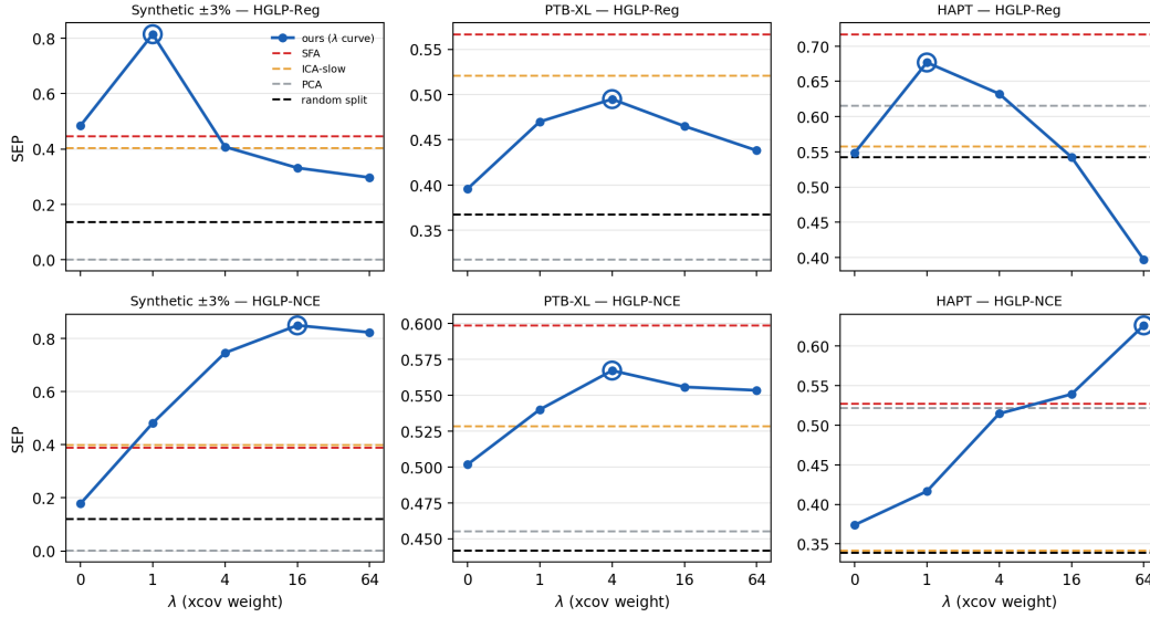
Figure 5: SEP against the penalty weight \lambda . n = 5 seeds. Our method traces a curve over \lambda \in \{0, 1, 4, 16, 64\} with its best point ringed; each post-hoc unmixing has no knob and is a horizontal line. A win is our curve rising above the SFA line. Unlike an inclusion–exclusion plane, this view combines all three SEP terms, so it also shows the one real-data win, which the inclusion–exclusion plane cannot display.
