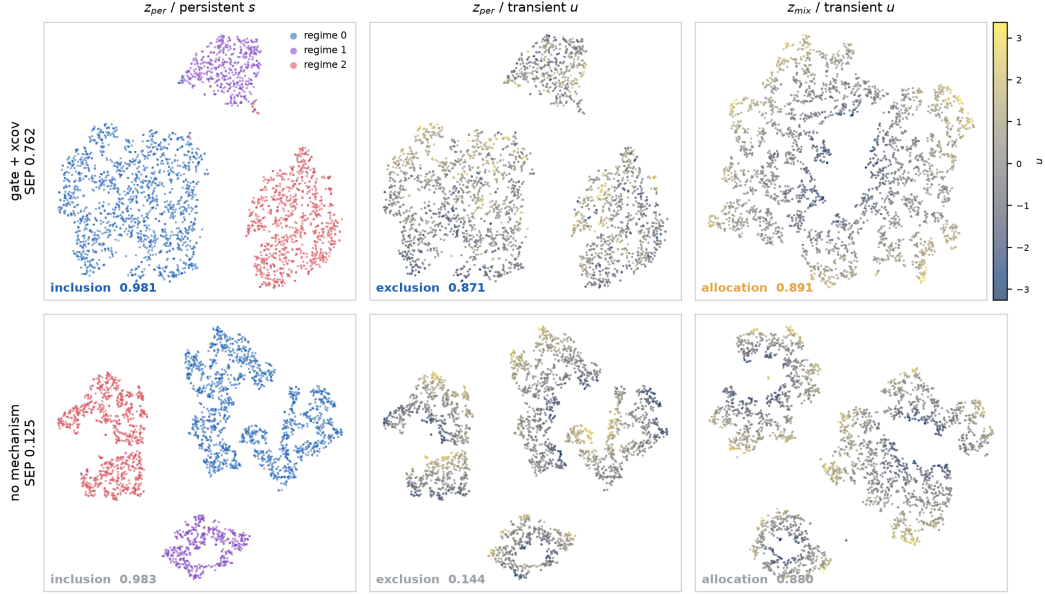
Figure 4: The three terms of SEP, with and without the mechanism. A t-SNE of one block per panel (synthetic \pm 3\% , HGLP-NCE, \lambda = 4 , one seed), coloured by one factor; the columns are exactly the three terms of Eq. 6 and the bottom row is a model trained with no gate, no penalty and no per-block LayerNorm. Each panel carries its term’s value, and the whole gap between the rows is one column : inclusion is 0.981 against 0.983 and allocation 0.891 against 0.880, both unchanged, while exclusion is 0.871 against 0.144 — SEP 0.762 against 0.125. The left column is therefore not a result: the regimes separate in z_{\text{per}} either way, as the random-subspace control above already said. What our devices change is the middle column. Read it by the colour scale rather than by eye, since the difference between a partly ordered and a fully scrambled scatter is exactly what a linear probe sees and a reader does not. The fourth combination, z_{\text{mix}} coloured by the persistent factor, is not a term of SEP and is unconstrained by design (Section 3.2), so it is omitted.
