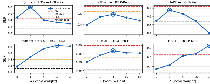
Figure 4: SEP against the penalty weight \lambda , n = 5 seeds. Our method traces a curve with its best point ringed; each post-hoc unmixing has no knob and is a horizontal line. A win is our curve rising above the SFA line.
