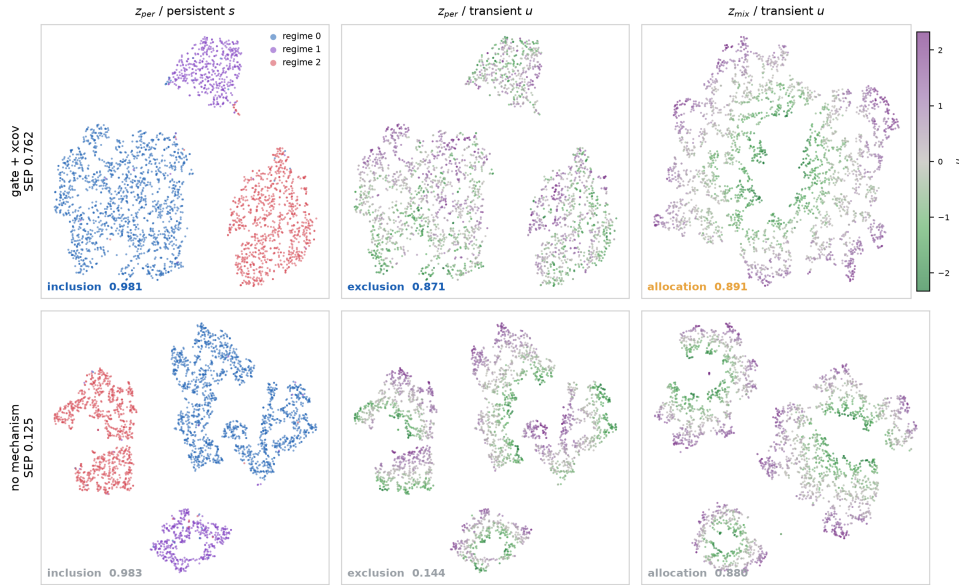
Figure 5: The exclusion term, seen directly. The two blocks against both factors, with and without the mechanism (synthetic \pm 3\% , HGLP-NCE, \lambda = 4 , one seed). The middle column is the only one that differs between the rows: inclusion is 0.981 against 0.983 and allocation 0.891 against 0.880. The fourth combination, z_{\text{mix}} against the persistent factor, is not a term of SEP and is unconstrained by design, so it is omitted.
