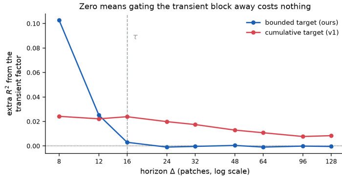
Figure 4: R^2(s, u \rightarrow \bar{z}_{t+\Delta}) - R^2(s \rightarrow \bar{z}_{t+\Delta}) : what the transient factor adds, beyond the persistent one, to a linear reading of the target embedding \Delta ahead. Zero means gating it away costs nothing. Synthetic, HGLP-Reg, 2,500 steps, one seed, ground-truth factors.
