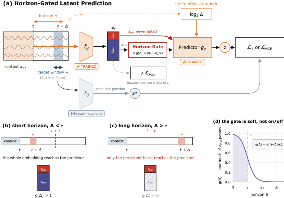
Figure 2: Horizon-gated latent prediction. (a) A causal encoder maps a window to z_t , split into z_{\text{per}} (16 of 64 dimensions) and z_{\text{mix}} ; a predictor conditioned on \Delta matches a target read at one position inside (t, t + \Delta] . (b, c) The same pipeline at a short and a long horizon. (d) The gate, with the axis in units of \tau .
