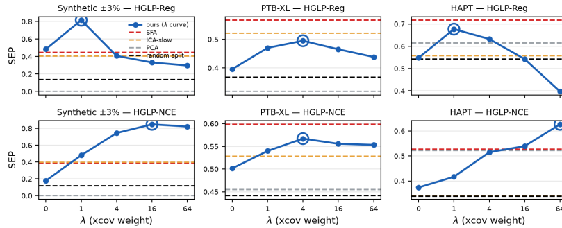
Figure 3: SEP against the penalty weight \lambda , n = 5 seeds. Our method traces a curve with its best point ringed; each post-hoc unmixing has no knob and is a horizontal line. A win is our curve rising above the SFA line.
