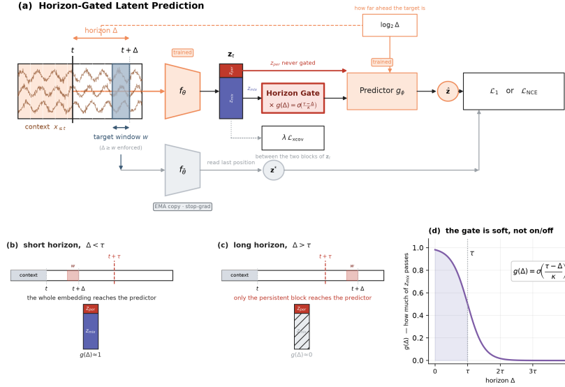
Figure 2: Horizon-gated latent prediction. (a) A causal encoder maps a window to z_t , split into z_{\text{per}} (16 of 64 dimensions) and z_{\text{mix}} ; a predictor conditioned on \Delta matches a target read at one position inside (t, t + \Delta] . (b, c) The same pipeline at a short and a long horizon. (d) The gate, with the axis in units of \tau .
