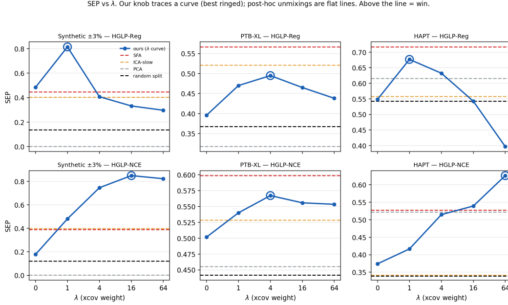
Figure 5: SEP against the penalty weight \lambda . n = 5 seeds. Our method traces a curve over \lambda \in \{0, 1, 4, 16, 64\} with its best point ringed; each post-hoc unmixing has no knob and is a horizontal line. A win is our curve rising above the SFA line. Unlike an inclusion–exclusion plane, this view combines all three SEP terms, so it also shows the one real-data win, which the inclusion–exclusion plane cannot display.
