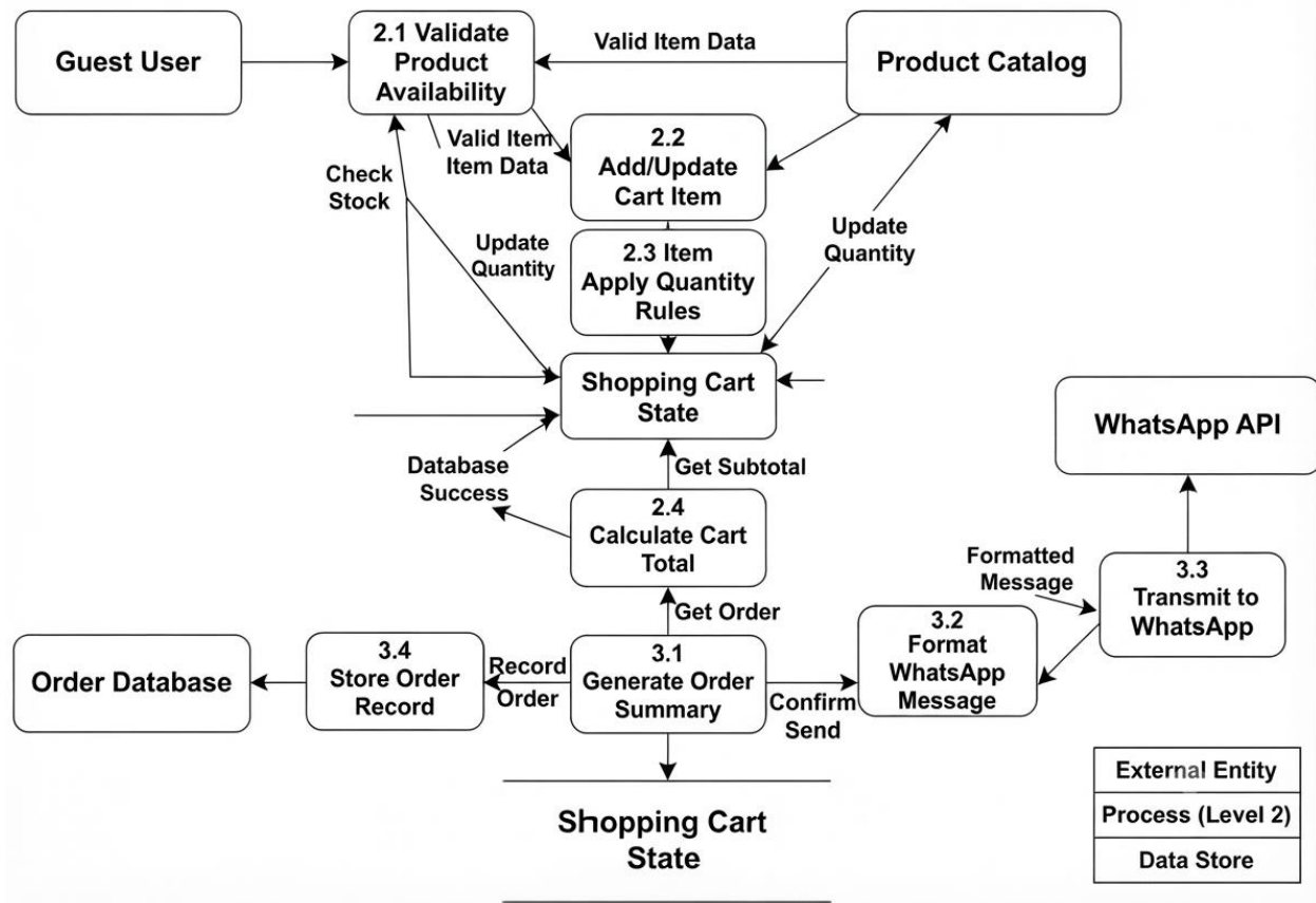
Level 2 DFD: Detailed Shopping Cart & Order Process
