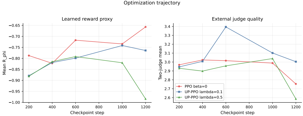
Figure 1: Optimization trajectory. PPO exhibits late proxy improvement with judge degradation; UP-PPO \lambda = 0.1 sacrifices some proxy reward for better external quality.
