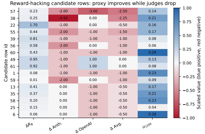
Figure 3: Reward-hacking candidate rows. Blue indicates positive change and red indicates negative change from PPO step 1000 to step 1200.
