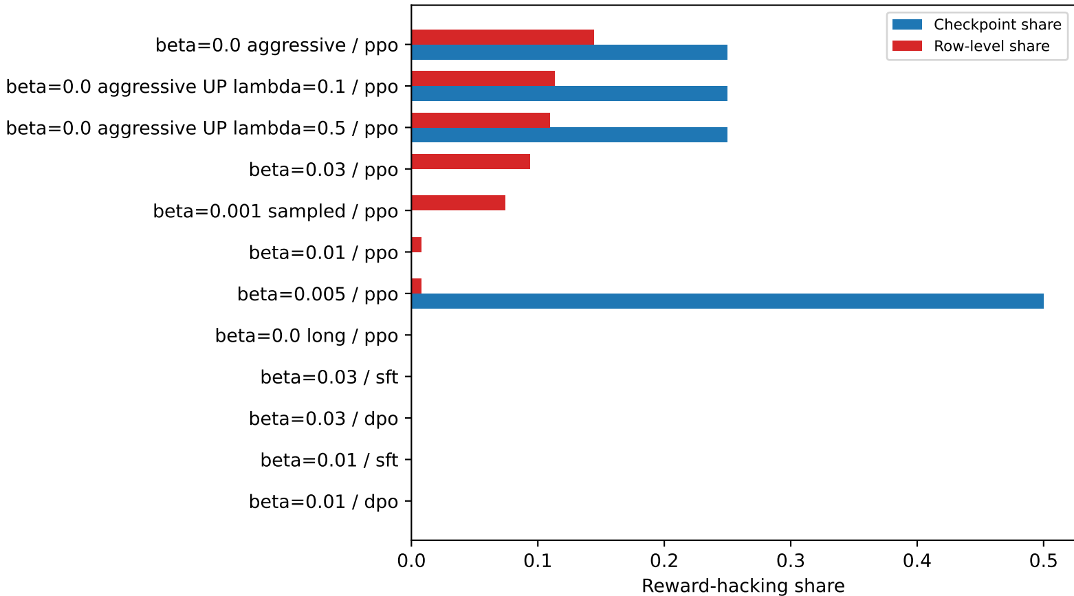
Ablation: Aggregate Checkpoints vs Row-Level Diagnostics
