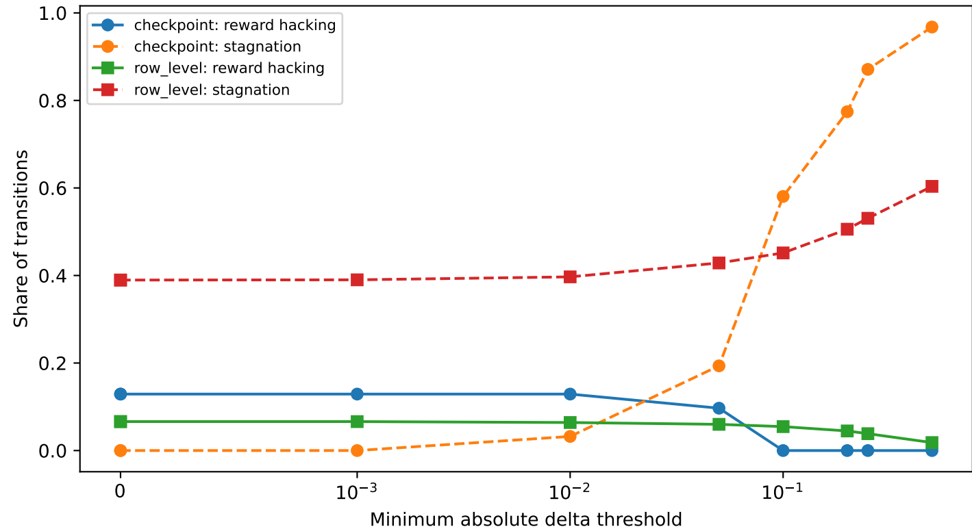
Taxonomy Sensitivity to Effect-Size Threshold
