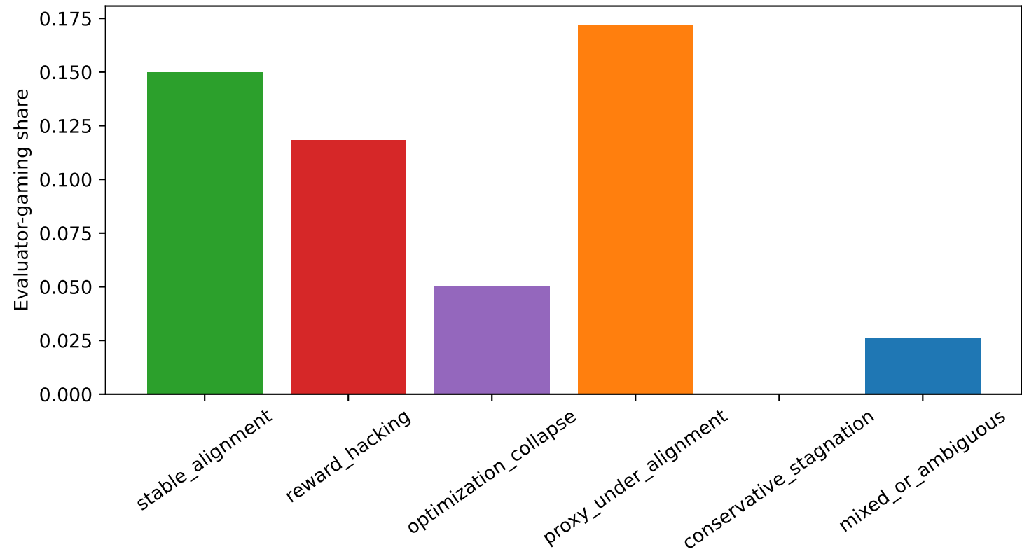
Judge Disagreement Concentrates by Failure Mode
