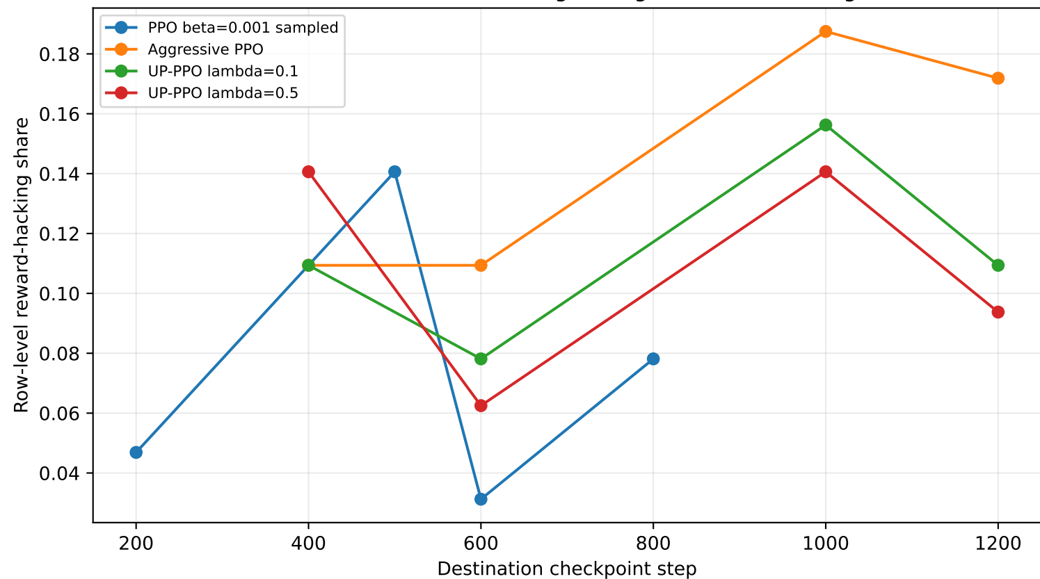
Localized Reward-Hacking Emergence Over Training
