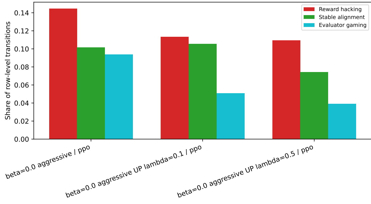
Aggressive PPO vs UP-PPO Failure-Mode Shares
