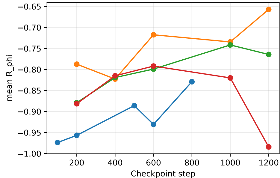
Reward uncertainty trajectory
