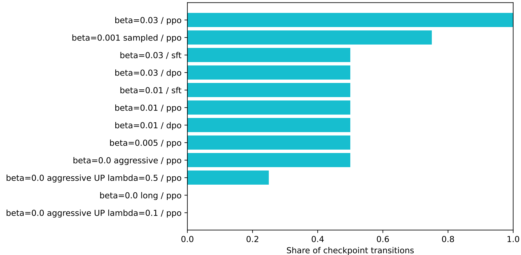
Evaluator-Disagreement Events by Setting
