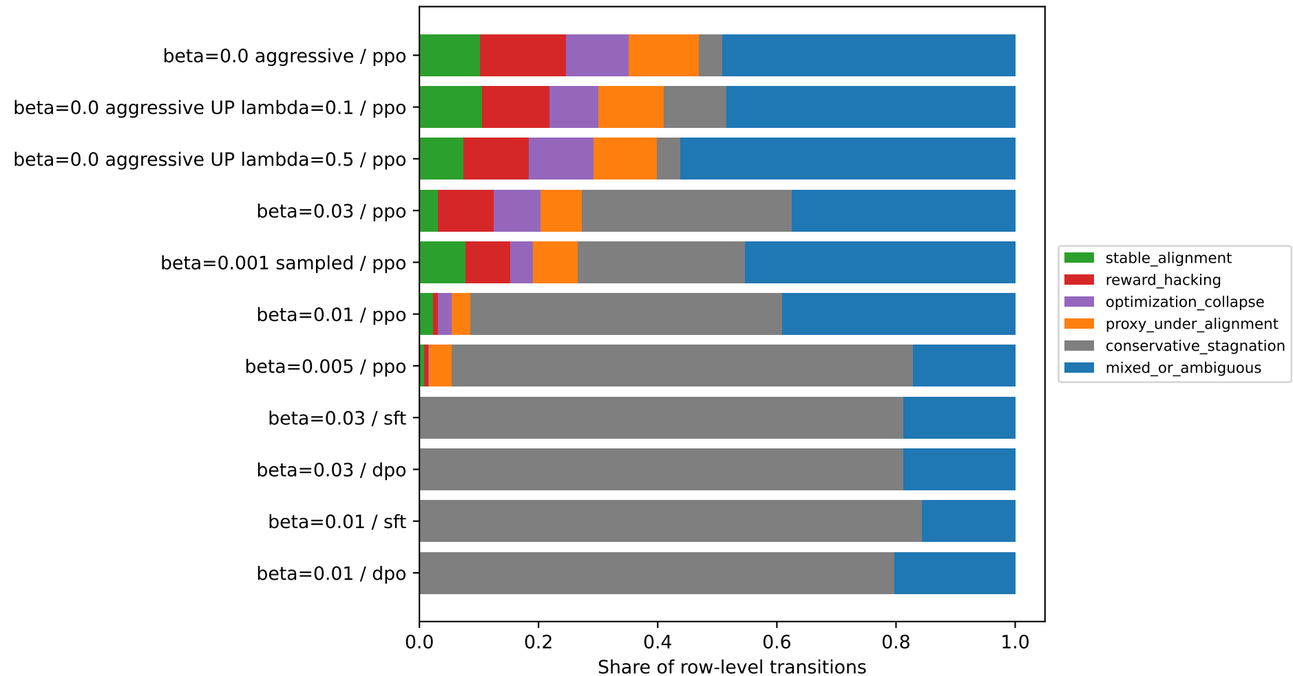
Row-Level Failure Modes Reveal Localized Failures
