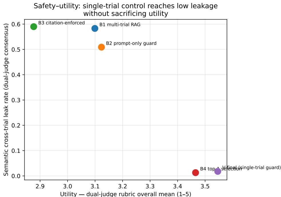
Figure 5: Safety–utility trade-off across systems. x -axis: dual-judge-pooled rubric overall mean (baselines pooled over Sonnet 4.5 + GPT-4o; V-final over the full n = 114 regime). y -axis: dual-judge-consensus semantic leak rate. Only the structural single-trial systems (B4, V-final) reach the low-leak region; B4 attains the highest utility among the four baselines.
