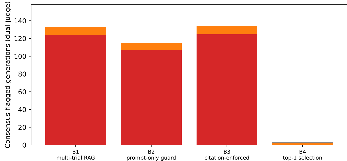
Failure taxonomy by system: structural control removes T1, not T2/T3
