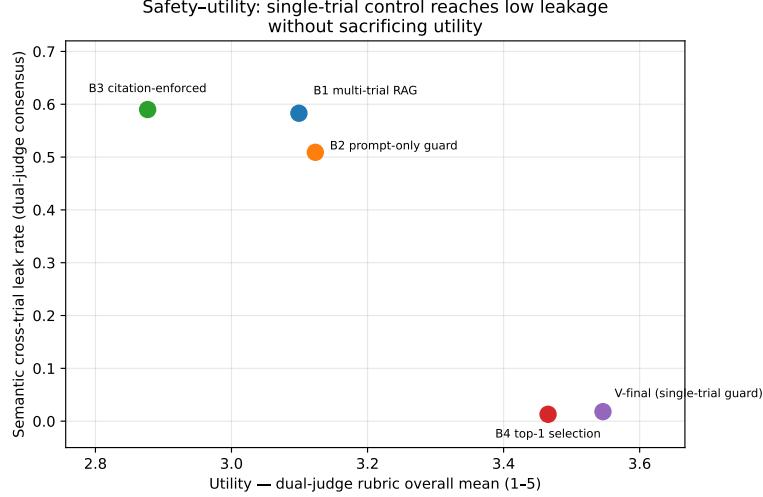
Fig. 5: Safety–utility trade-off across systems. x -axis: dual-judge-pooled rubric overall mean (baselines pooled over Sonnet 4.5 + GPT-4o; V-final over the full n = 114 regime). y -axis: dual-judge-consensus semantic leak rate. Only the structural single-trial systems (B4, V-final) reach the low-leak region.
