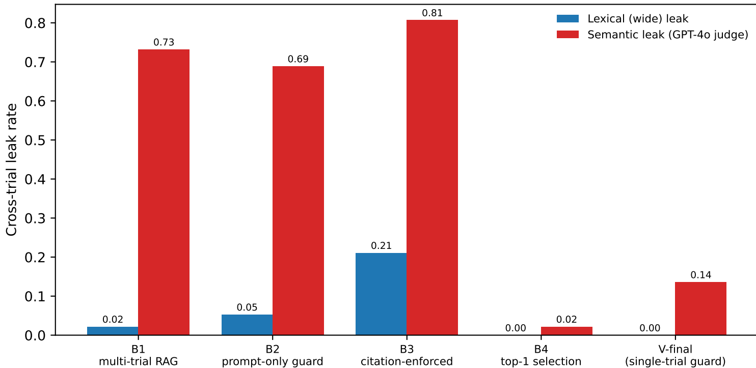
Cross-trial leakage by system: structural single-trial control vs alternatives
