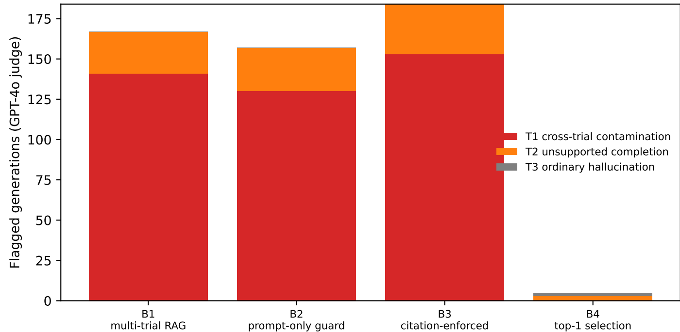
Failure taxonomy by system: structural control removes T1, not T2/T3
