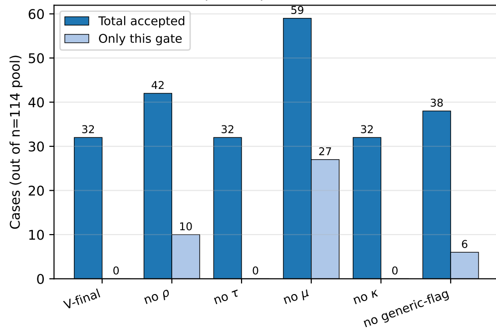
Selector acceptance per leave-one-out variant
