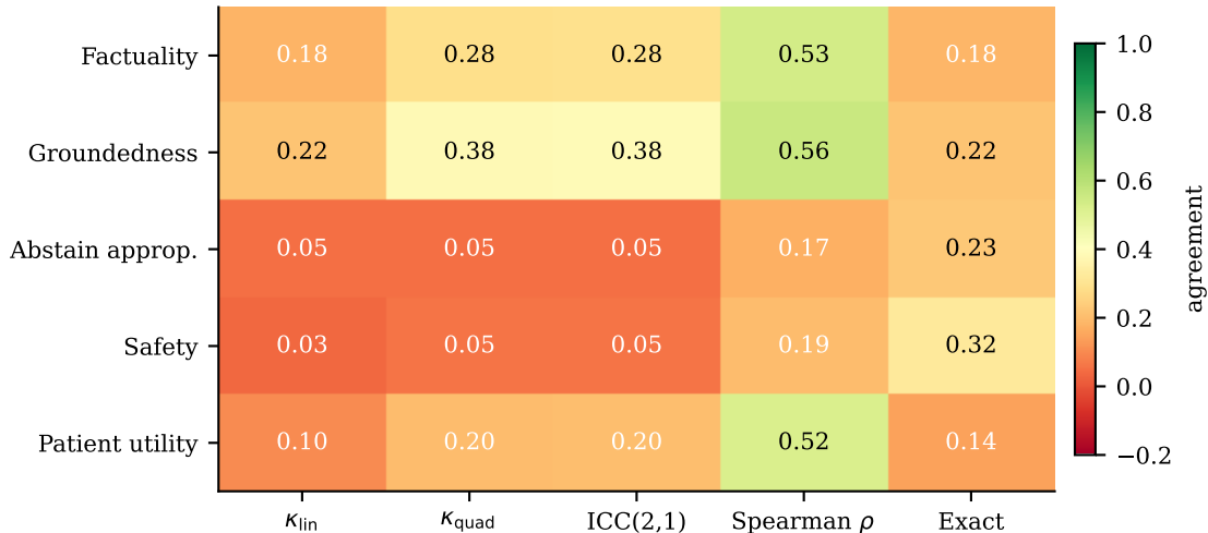
Sonnet-4 vs GPT-4o inter-rater agreement per rubric dim
