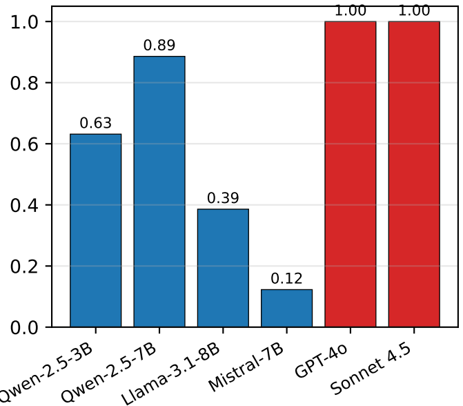
Parse OK rate
