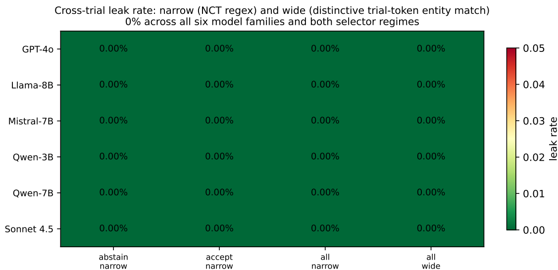
Figure S9: Per-(model × regime × definition) cross-trial leak rate. Rows: model family. Columns: selector regime × leak definition. Narrow = NCT-identifier regex; wide = identifier regex plus distinctive non-stop trial-token entity match. All cells are zero. The wide definition is strictly more permissive than the narrow one; their identical rates indicate the system does not emit narrative cross-trial references either. Demoted from main paper Fig. 2 (per peer-review feedback: an all-zero grid carries no visual information beyond what Table 1 already conveys); retained here for completeness.
