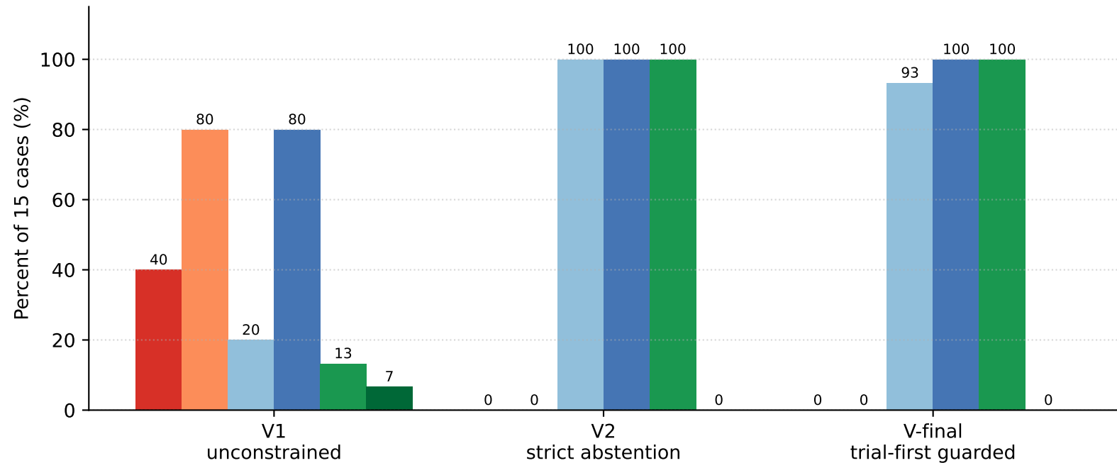
Safety-utility trade-off across three pipeline configurations
