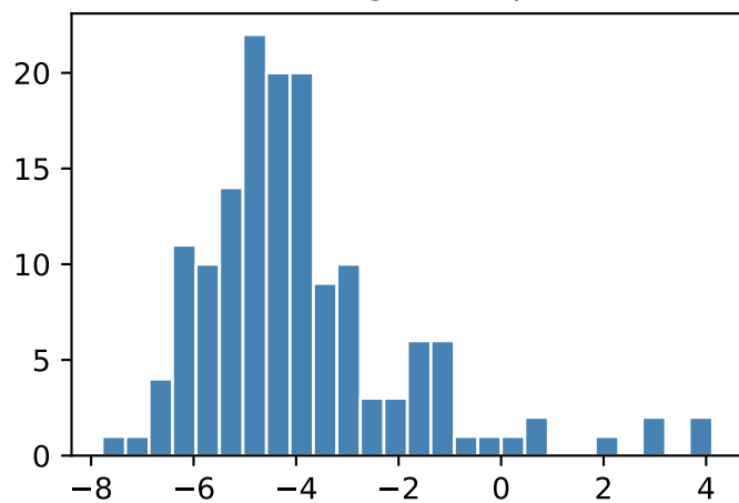
Histogram of \mu
