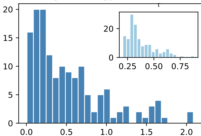
Histogram of \log \rho (n=150 cache)
