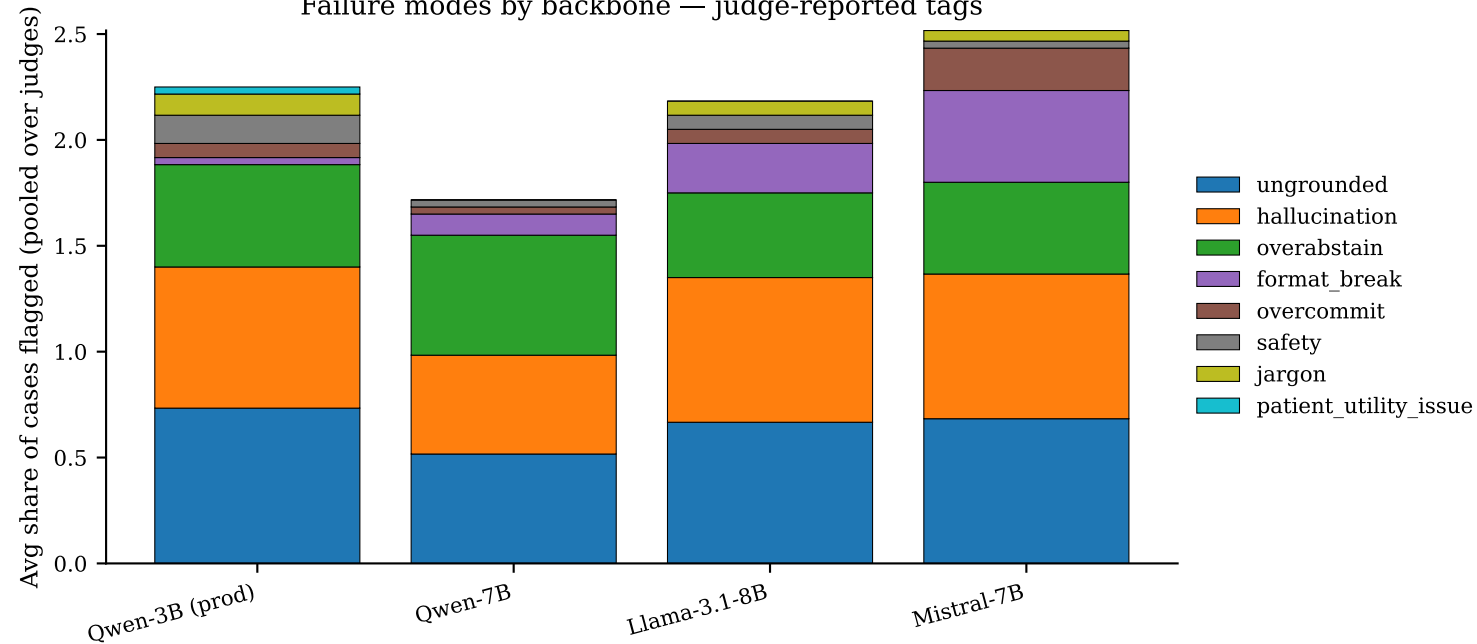
Failure modes by backbone — judge-reported tags
