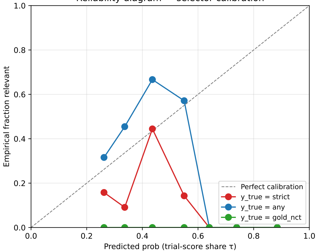
Reliability diagram — selector calibration
