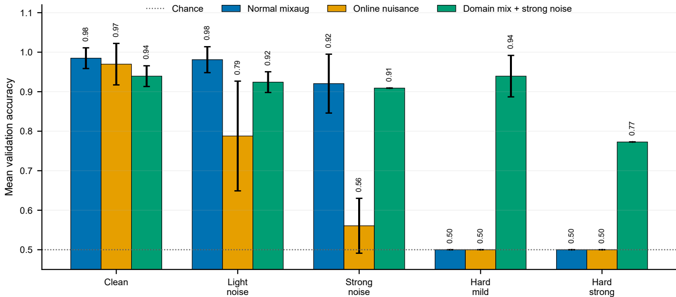
Training strategy comparison under noise and hard nuisance shifts
