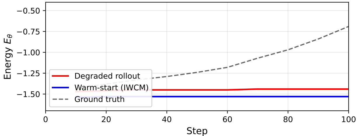
Recovery from degraded rollout (DM Control cartpole)
