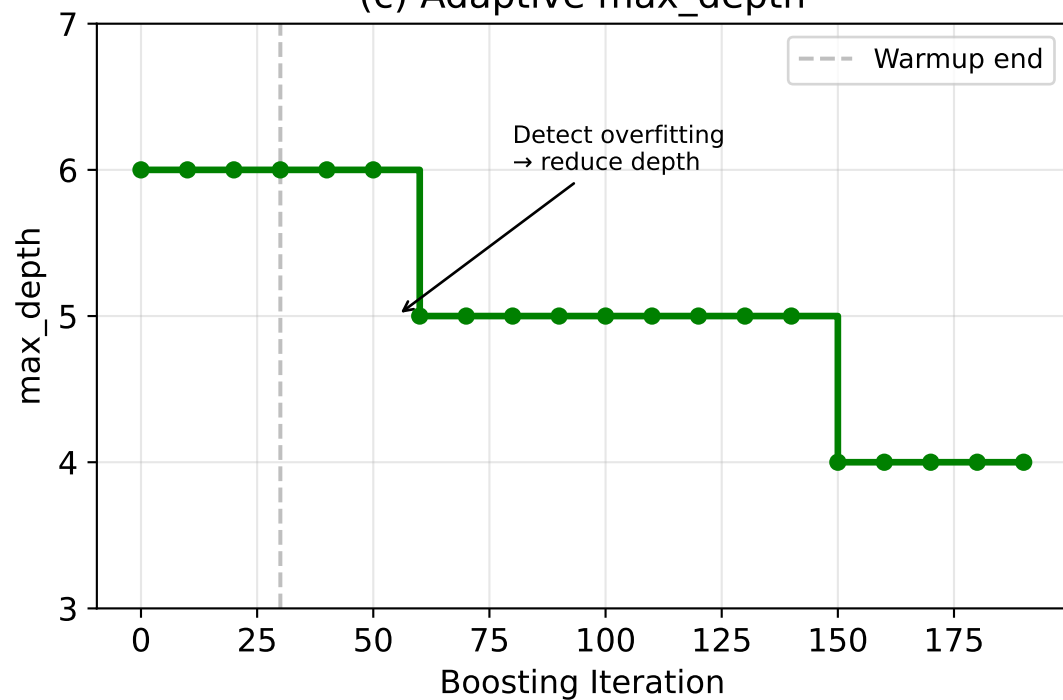
(c) Adaptive max_depth
