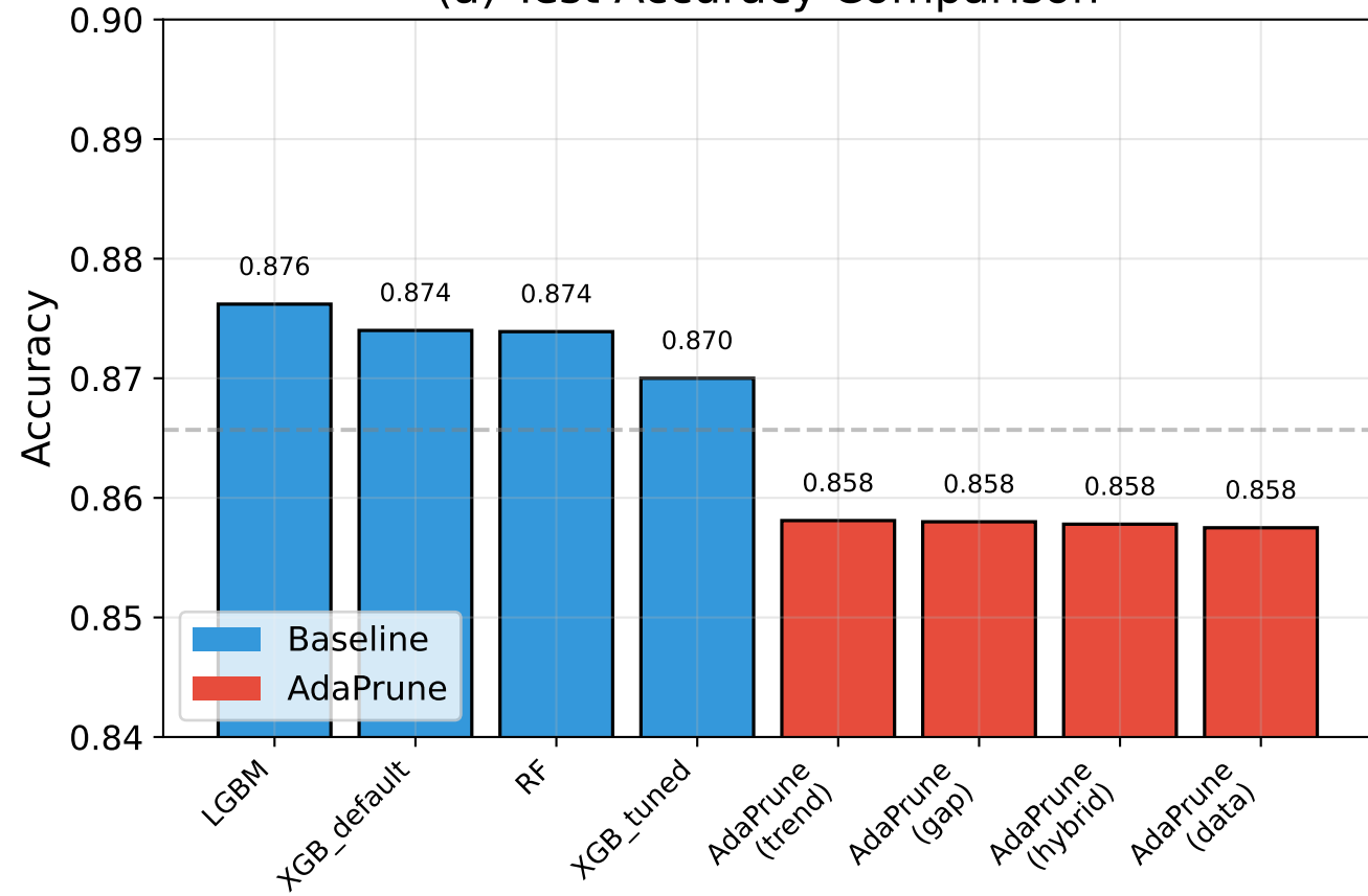
(a) Test Accuracy Comparison
