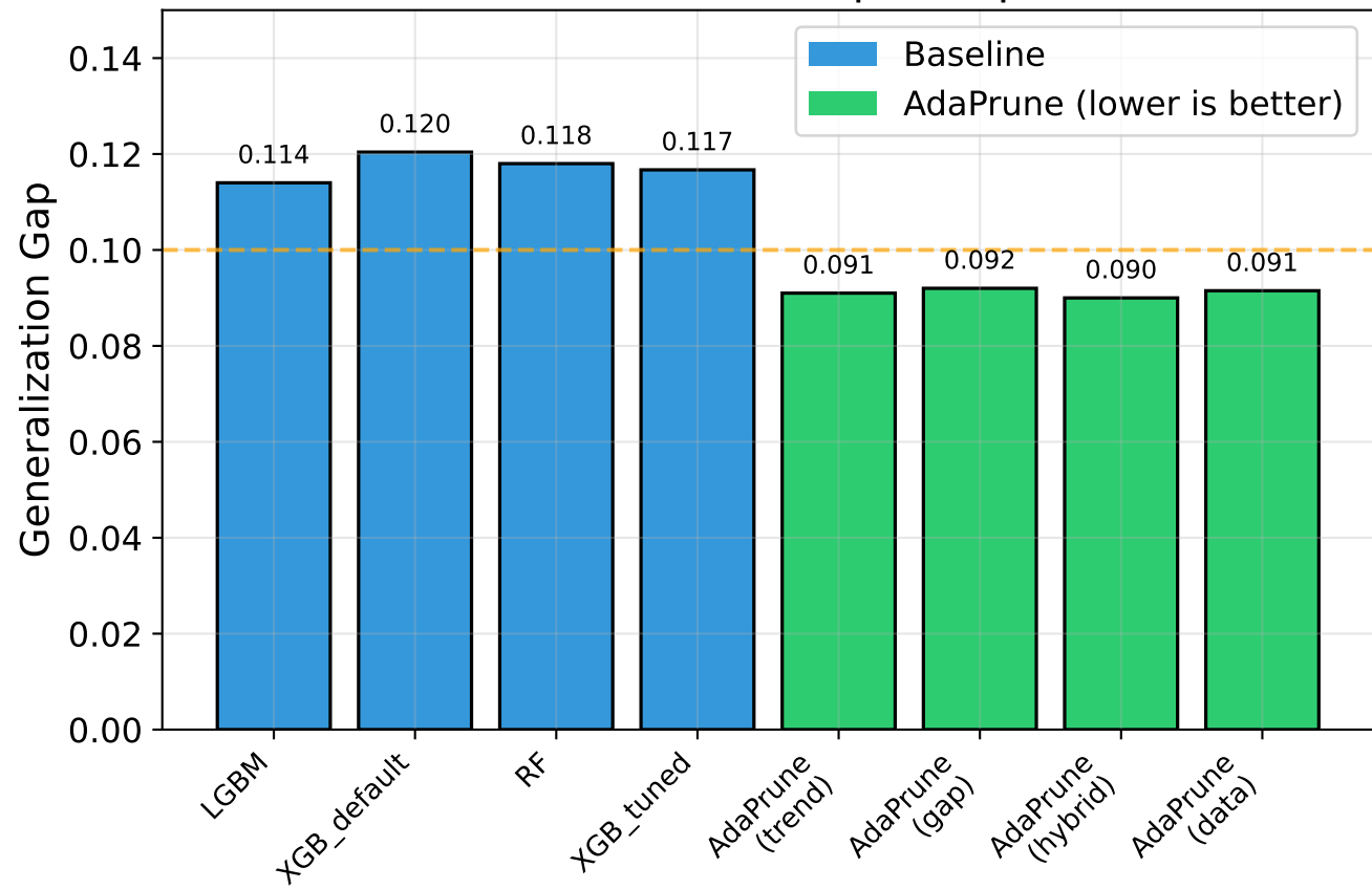
(b) Generalization Gap Comparison
