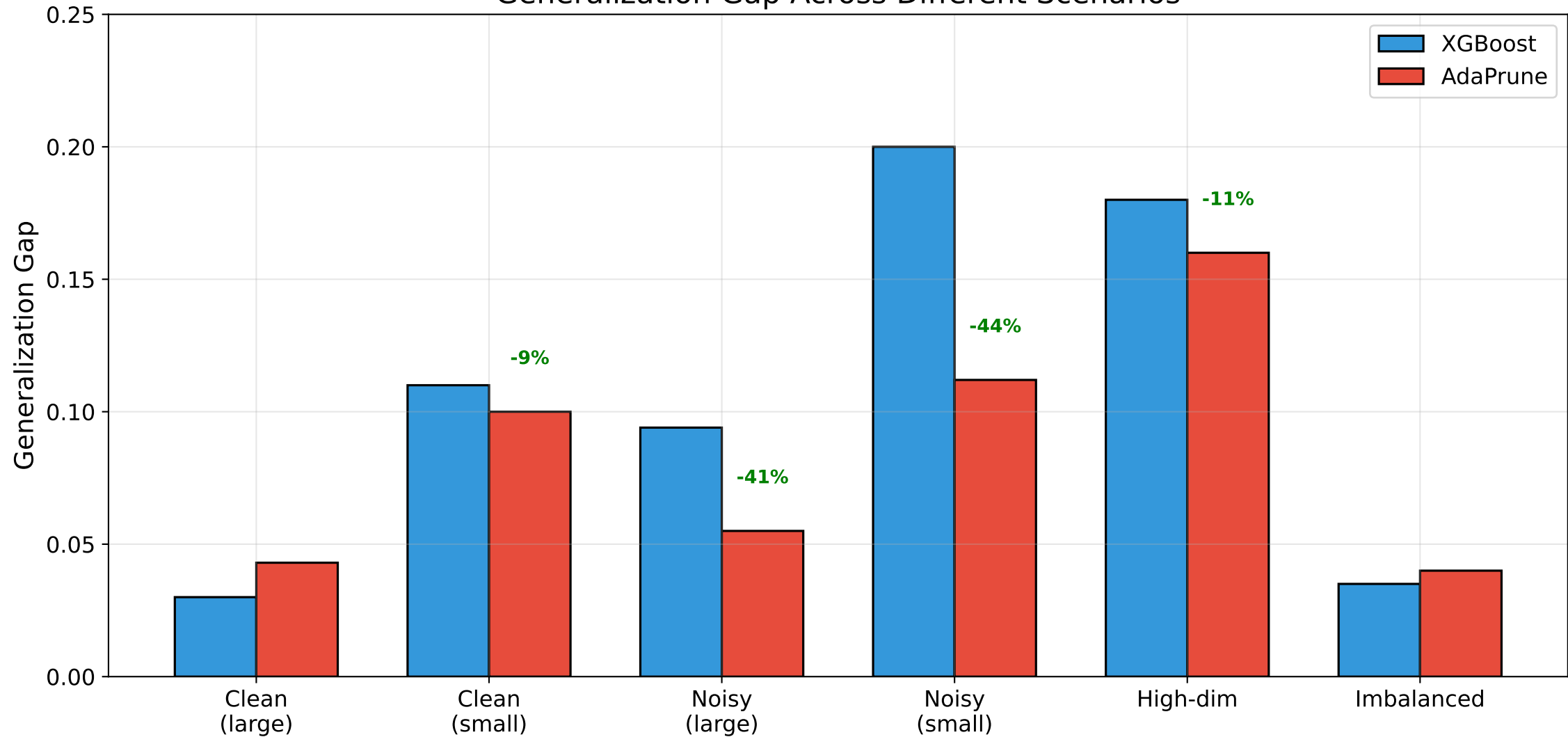
Generalization Gap Across Different Scenarios
