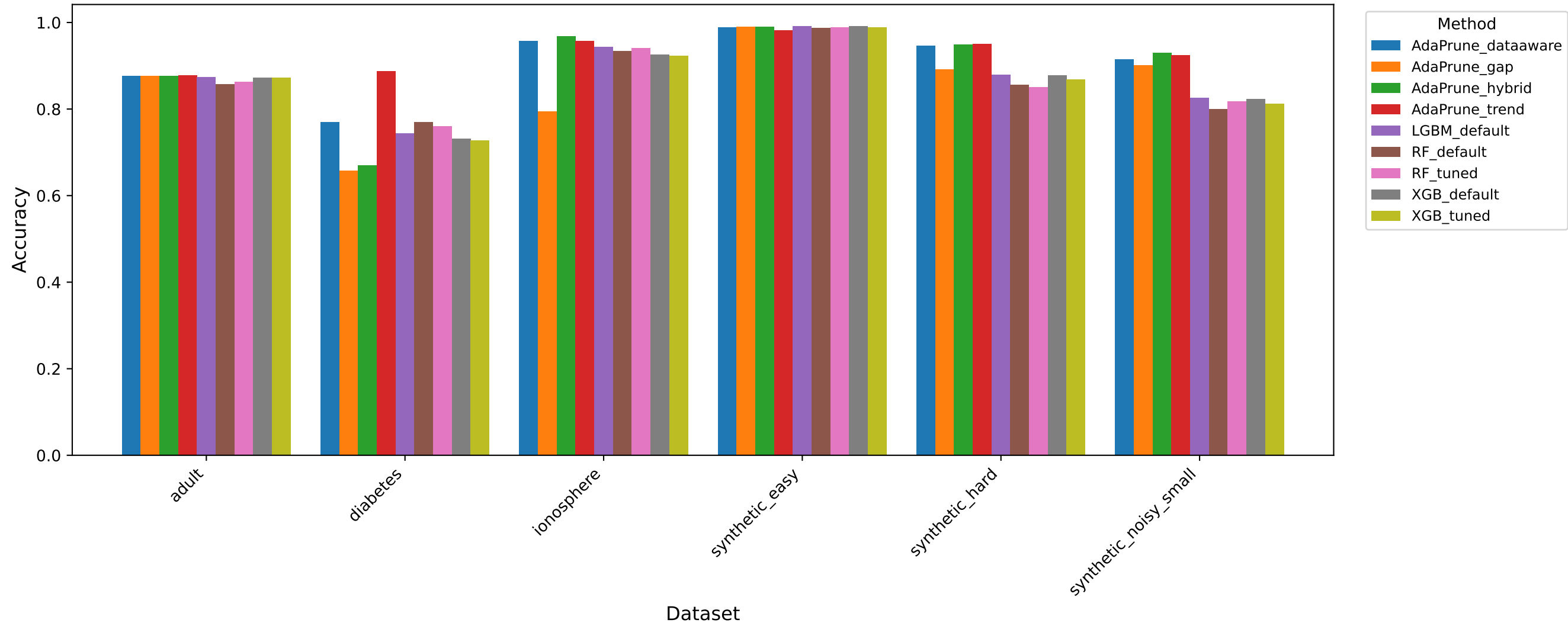
AdaPrune vs Baselines Comparison
