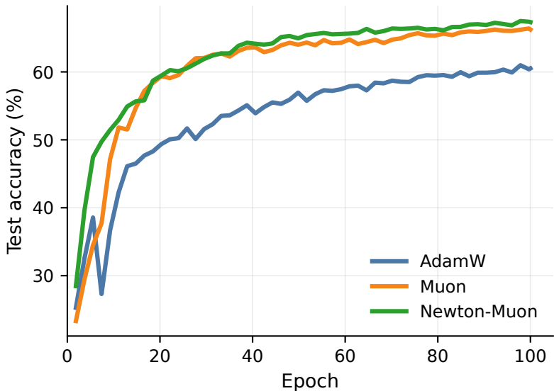
CIFAR-10 ResMLP-32
