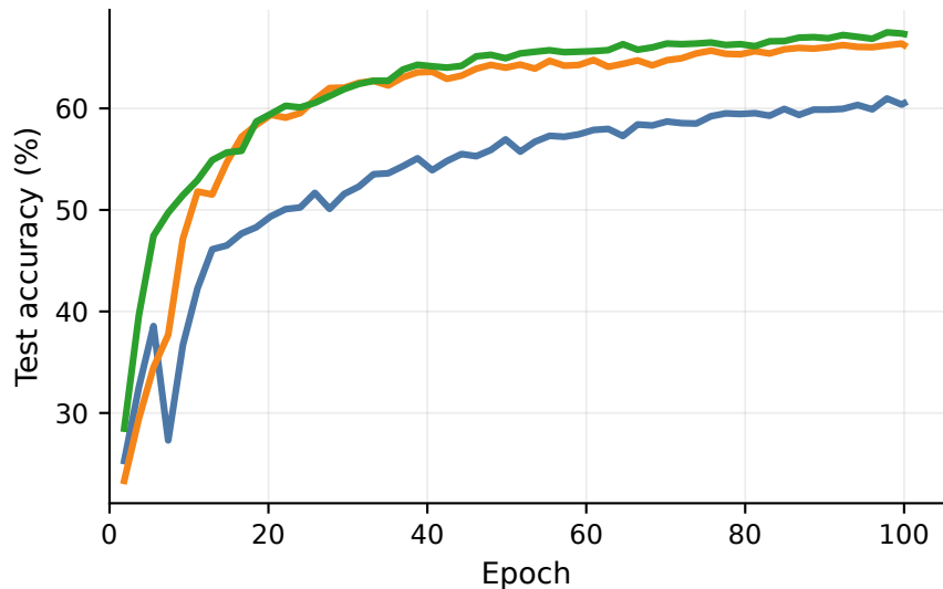
(a) CIFAR-10 ResMLP-32
